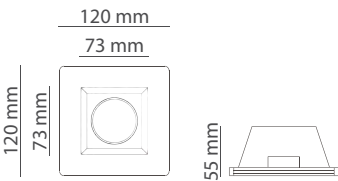
Dimensione foro 123x123 mm Cut hole sizes 123x123 mm
