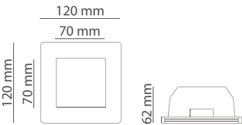
Dimensione foro 123x123 mm Cut hole sizes 123x123 mm
