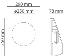
Dimensione foro 293x353 mm Cut hole sizes 293x353 mm
