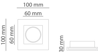
Dimensione foro 102x102 mm Cut hole sizes 102x102 mm
