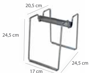
cod. RPB026A Rulliera porta bobina da pavimento per bobine tipo "A" Rolling coil carrier floor standing "A" type coils
